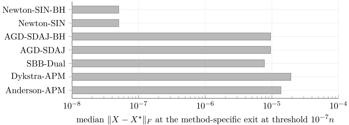
Figure 5: Achieved accuracy when each solver exits once its own stopping quantity reaches the threshold of the published dimension-scaled rule (tolerance 10^{-5} at n = 100 ; see table 15). Median forward errors range from 5.04 \times 10^{-8} (Newton variants) to 1.93 \times 10^{-5} (Dykstra-APM), a factor of 383. Costs measured at these exits are therefore costs at different accuracies.
