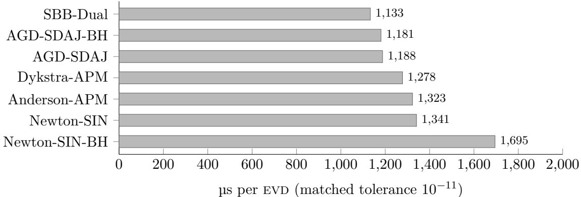
Figure 1: Median wall-clock time per EVD at n = 100 , all seven variants timed in one session. The spread is a factor of 1.50; Newton’s EVDs are the dearest, because they are accompanied by Krylov solves that the EVD count does not record. Anderson-APM’s EVDs cost 1.17 times SBB-Dual’s, the difference coming from its work outside the eigendecomposition, chiefly its least-squares update of O(mn^2) work per EVD.
