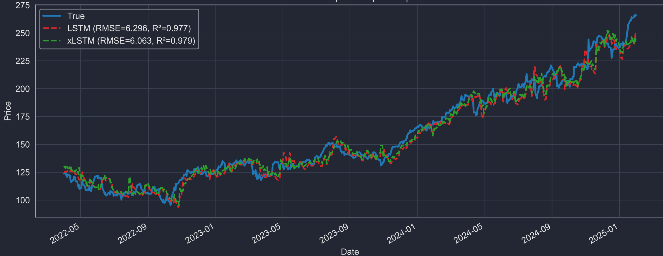
JPM – Prediction Comparison | H=10 | F=5 – TEST
