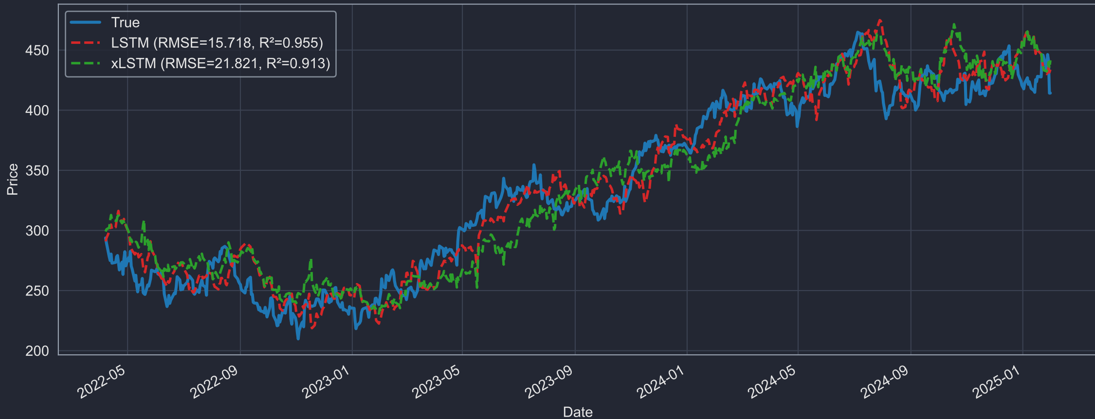
MSFT – Prediction Comparison | H=15 | F=5 – TEST
