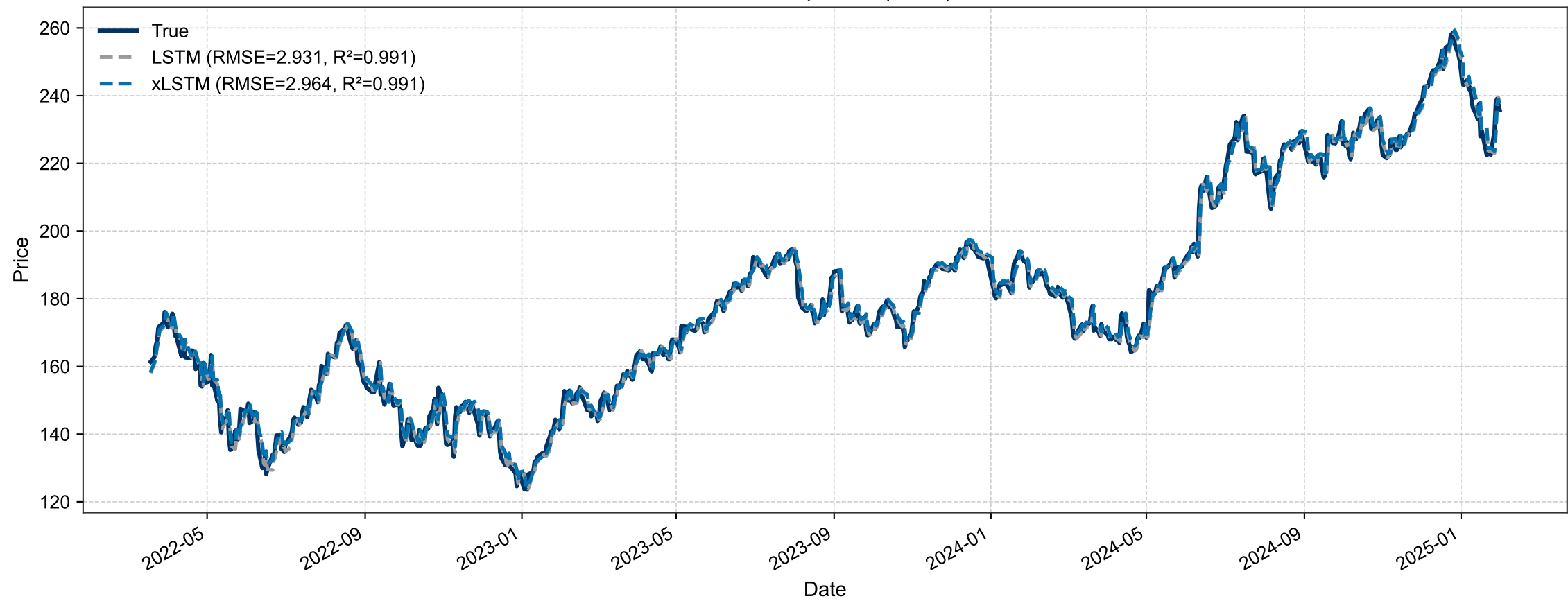
AAPL – Prediction Comparison | H=1 | F=1 – TEST
