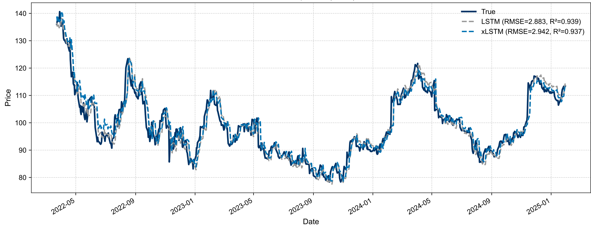
DIS – Prediction Comparison | H=3 | F=1 – TEST
