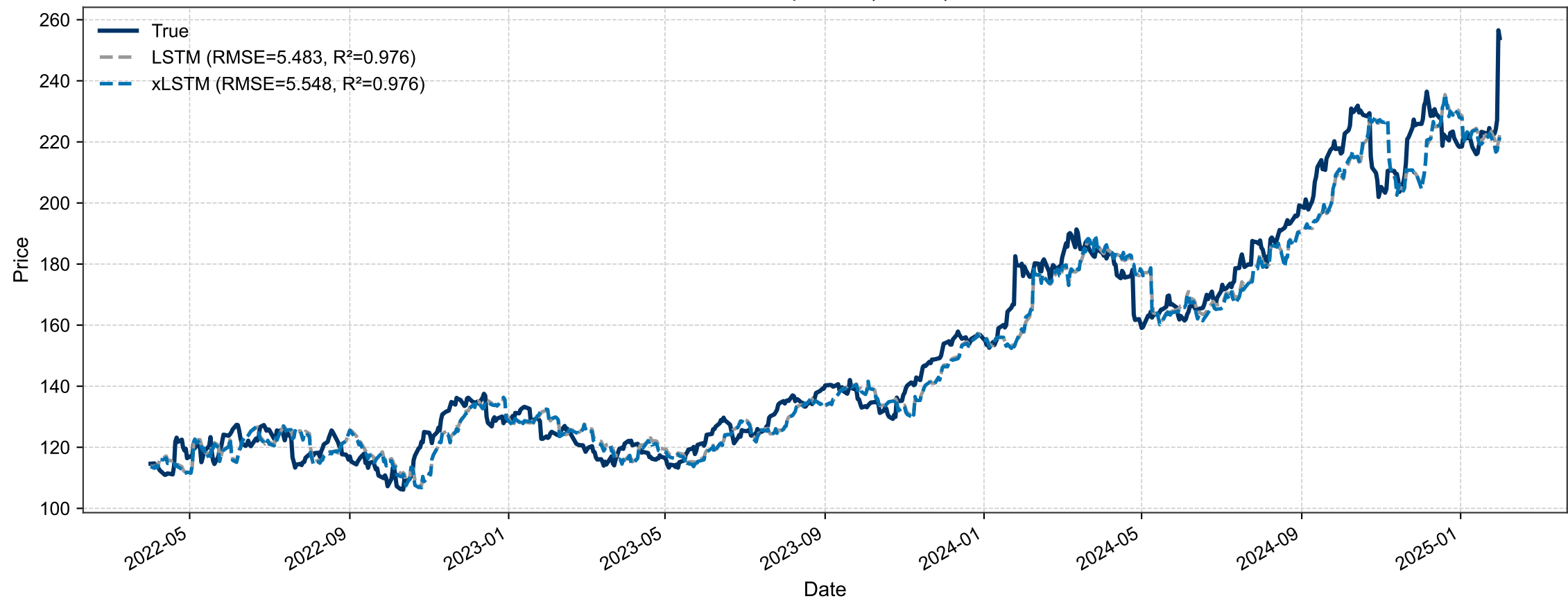
IBM – Prediction Comparison | H=10 | F=1 – TEST
