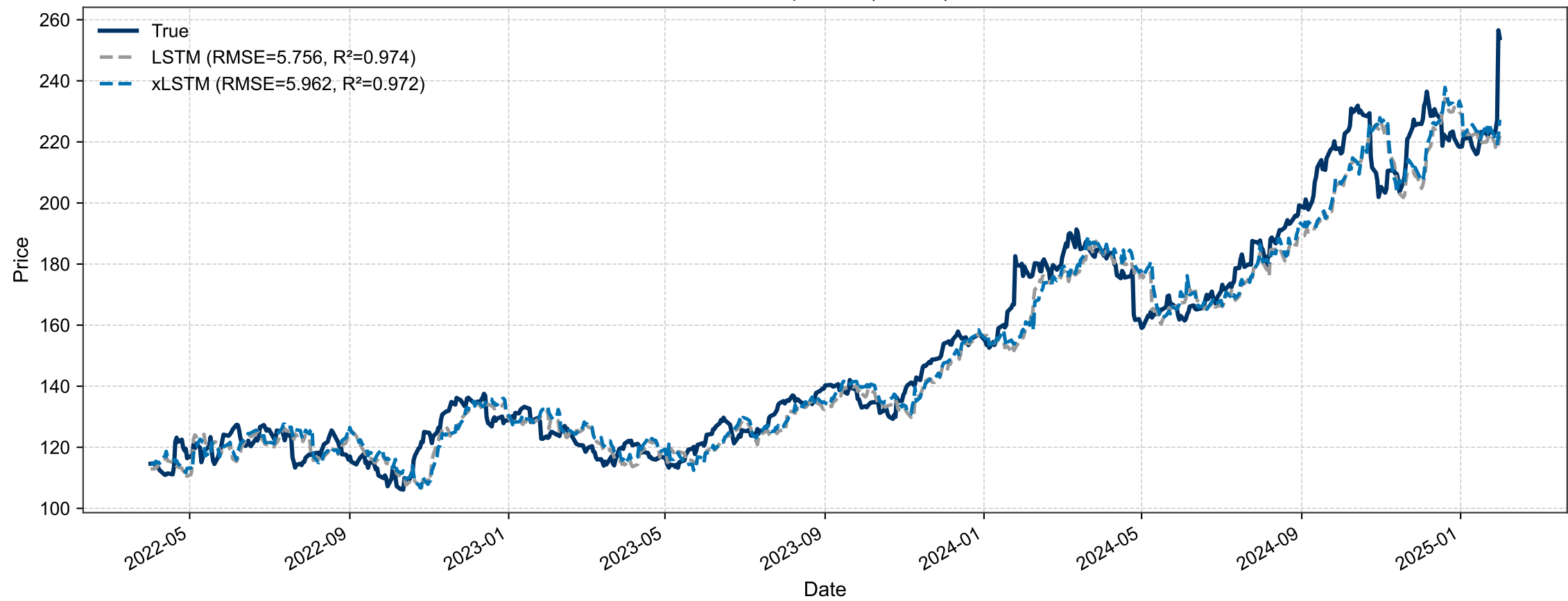
IBM – Prediction Comparison | H=10 | F=5 – TEST
