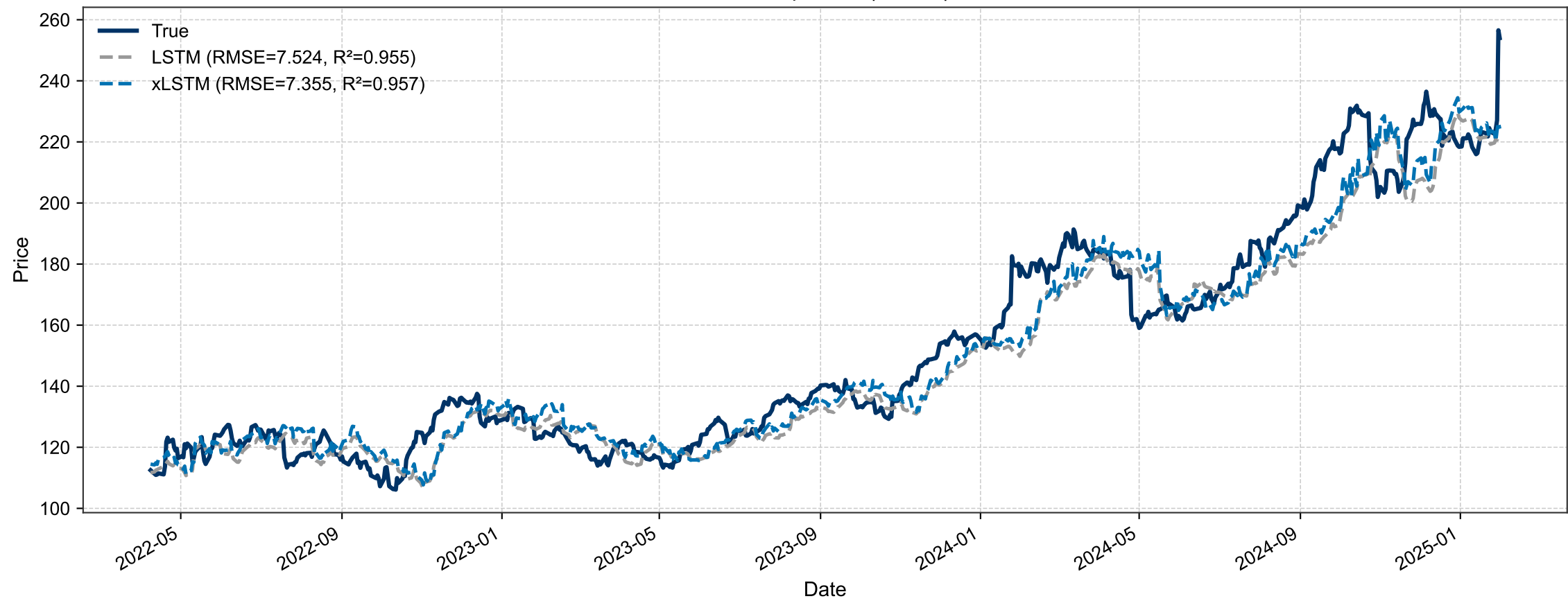
IBM – Prediction Comparison | H=15 | F=5 – TEST
