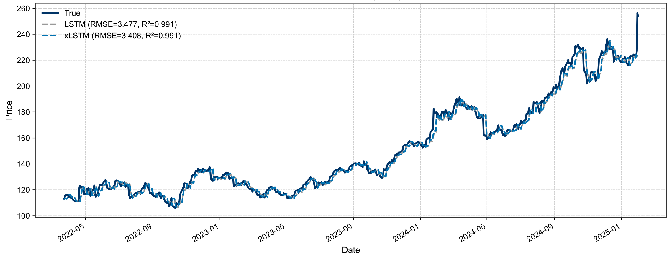
IBM – Prediction Comparison | H=3 | F=1 – TEST
