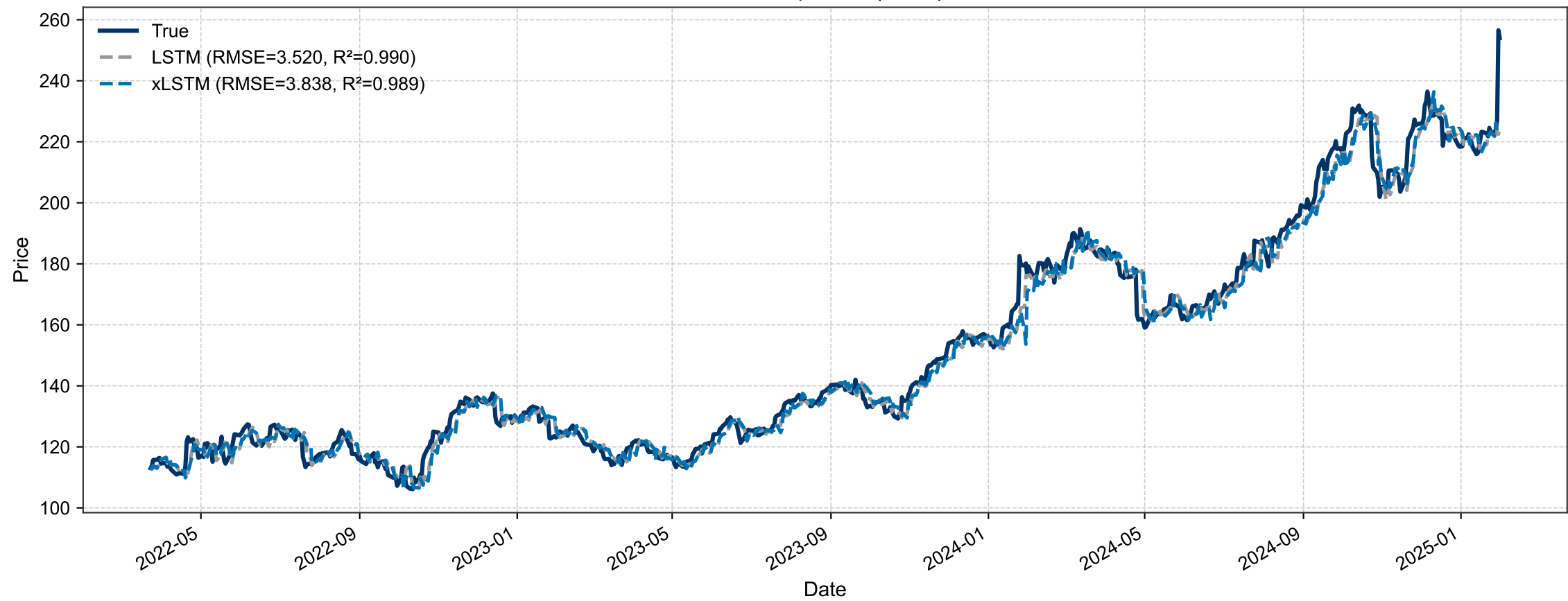
IBM – Prediction Comparison | H=3 | F=5 – TEST
