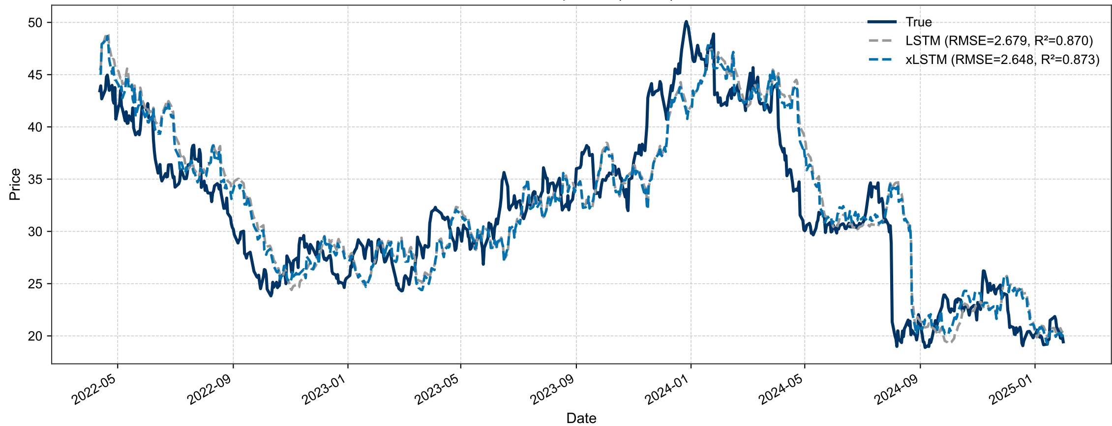
INTC – Prediction Comparison | H=15 | F=1 – TEST
