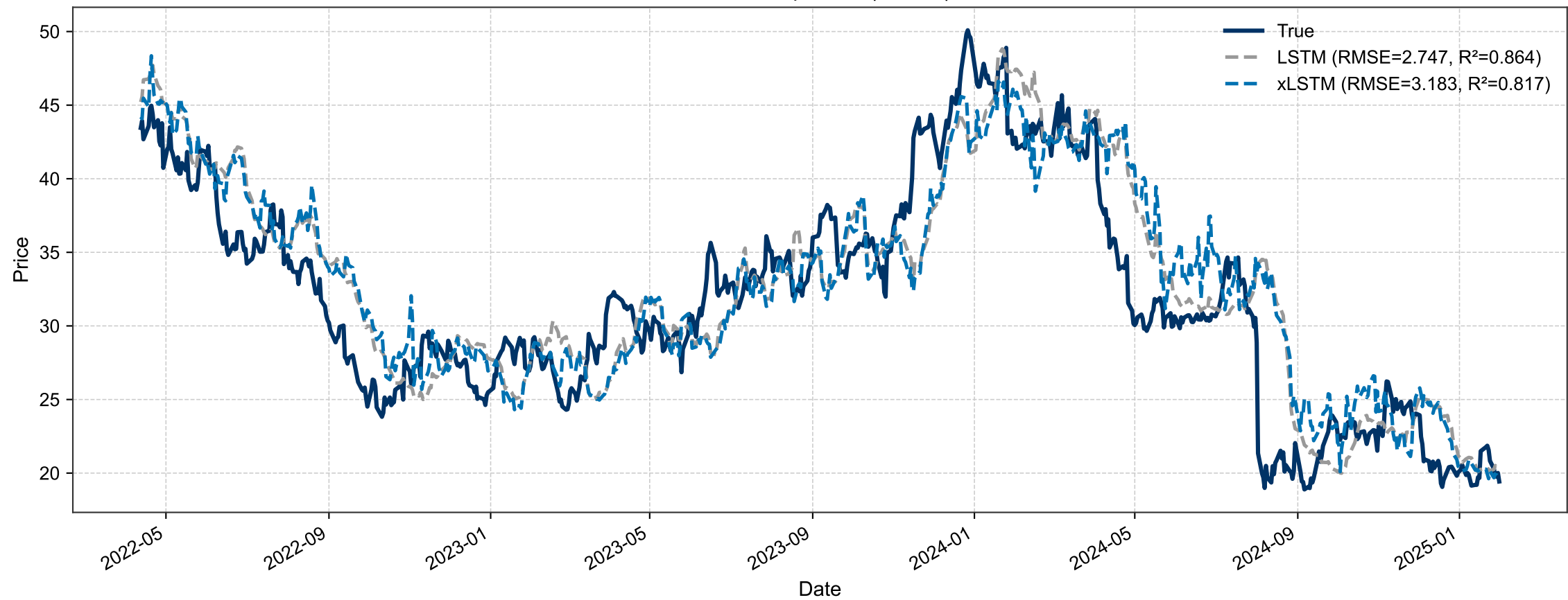
INTC – Prediction Comparison | H=15 | F=5 – TEST
