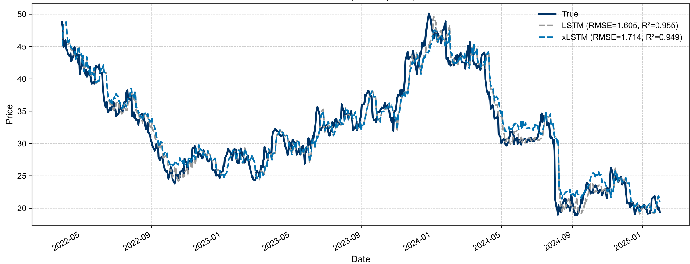
INTC – Prediction Comparison | H=5 | F=1 – TEST
