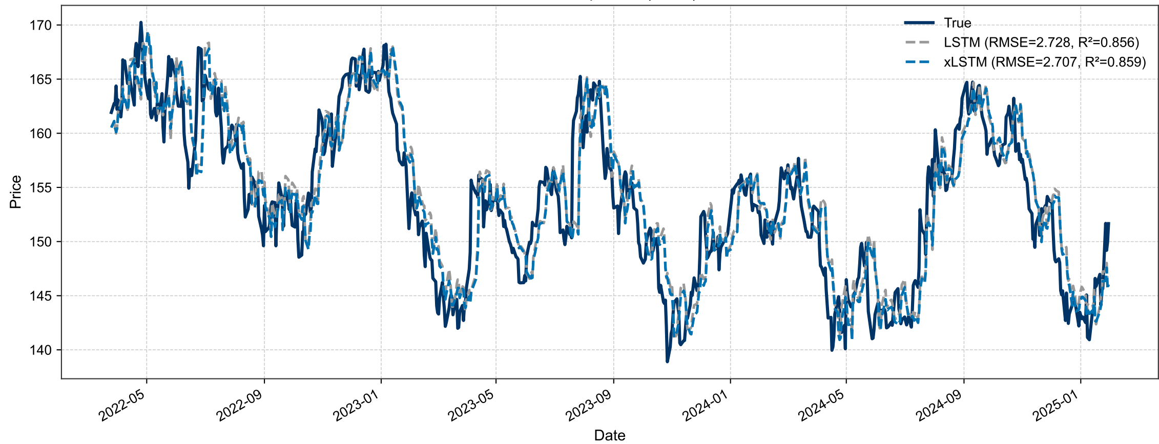
JNJ – Prediction Comparison | H=5 | F=1 – TEST
