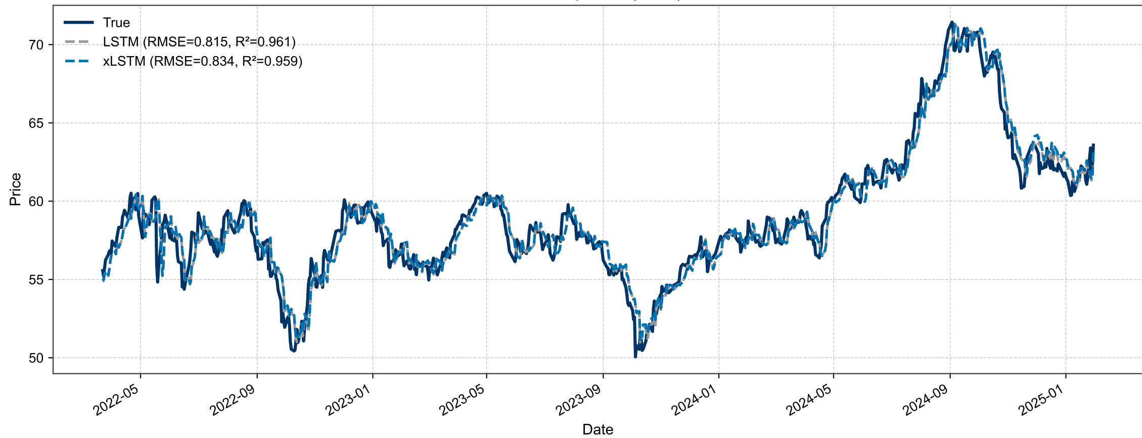
KO – Prediction Comparison | H=3 | F=1 – TEST
