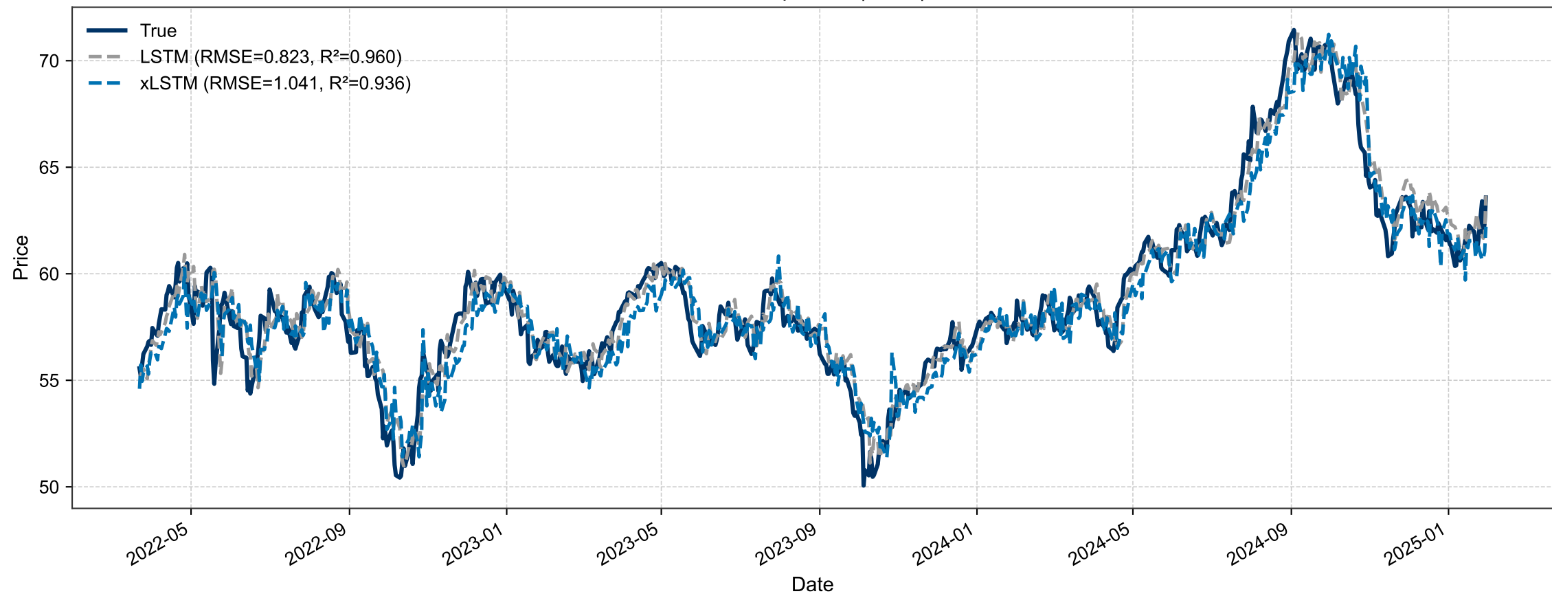
KO – Prediction Comparison | H=3 | F=5 – TEST
