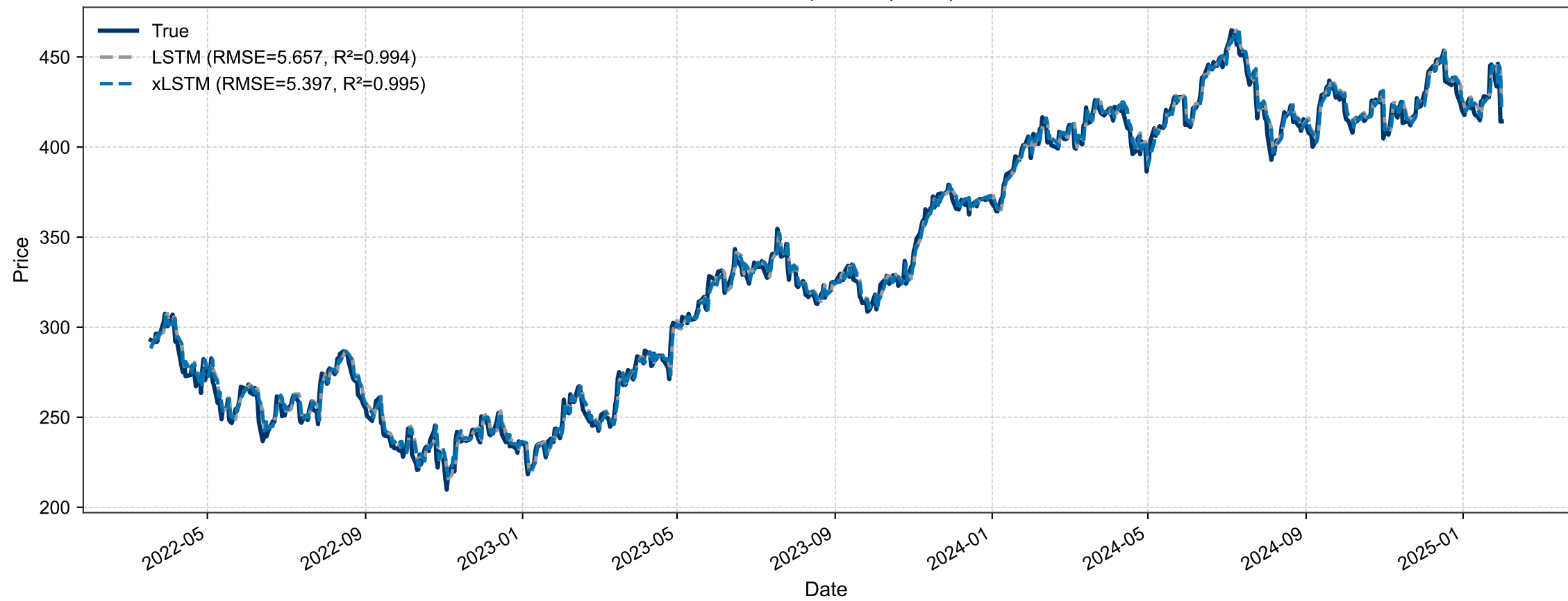
MSFT – Prediction Comparison | H=1 | F=1 – TEST
