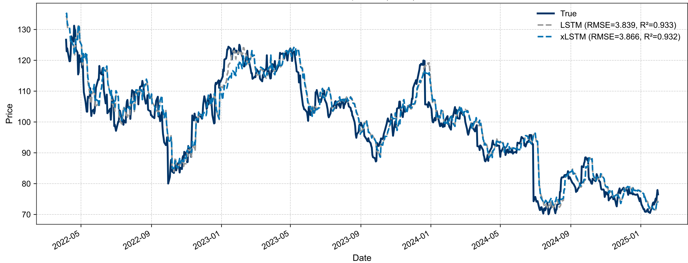
NKE – Prediction Comparison | H=5 | F=1 – TEST
