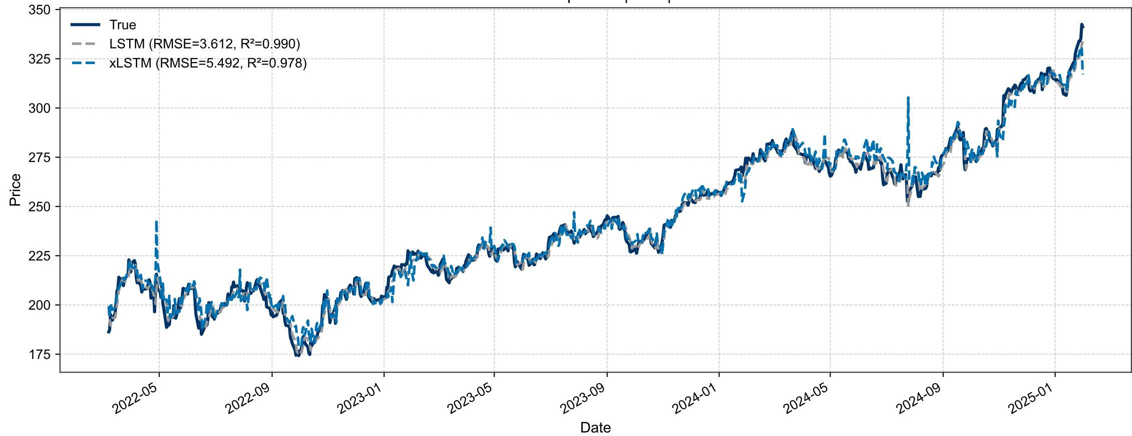
V – Prediction Comparison | H=1 | F=5 – TEST
