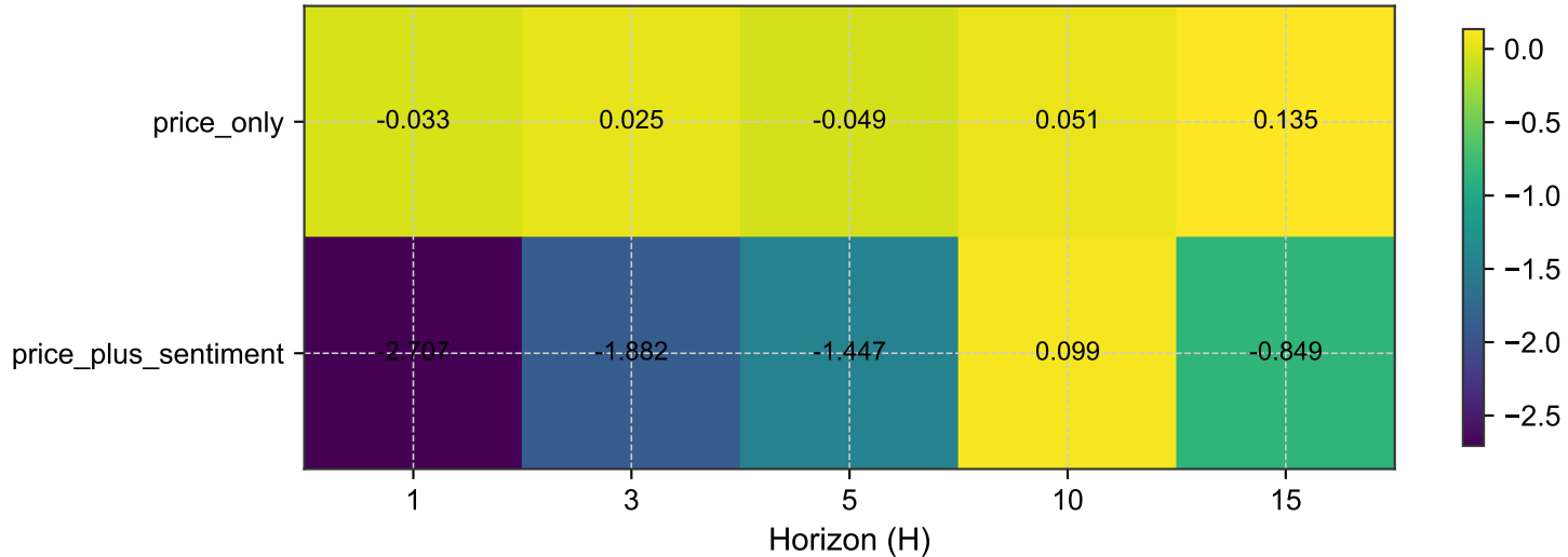
Error Reduction Heatmap – ER(RMSE) = RMSE(LSTM) - RMSE(xLSTM) (mean over assets)
