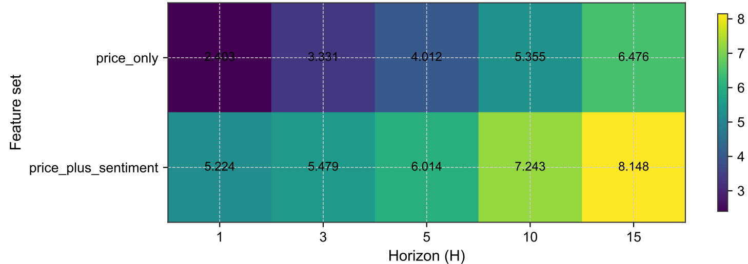
xLSTM – Heatmap RMSE (level, mean over assets)
