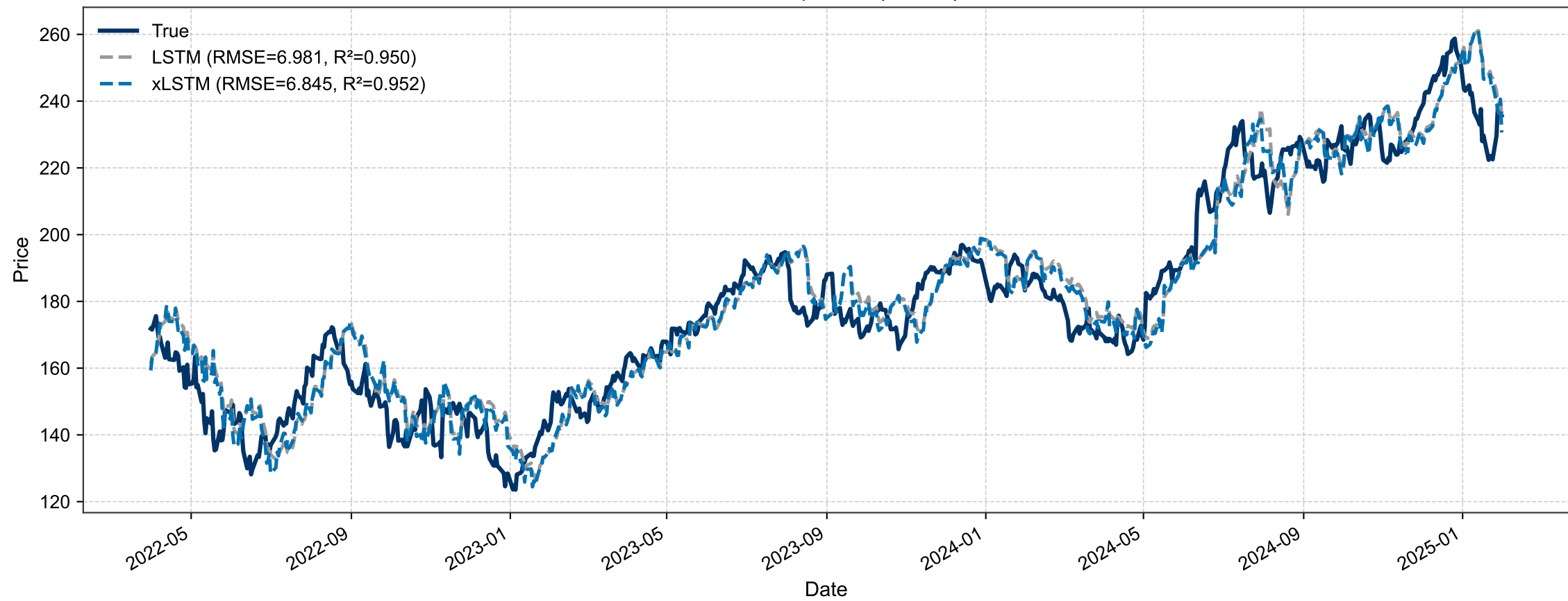
AAPL – Prediction Comparison | H=10 | F=1 – TEST
