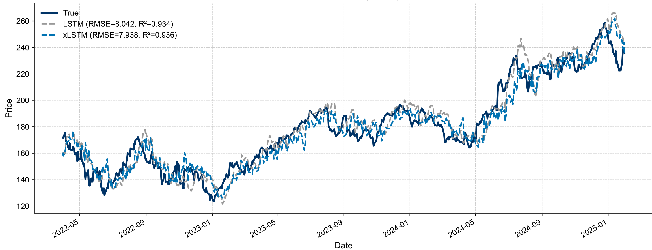
AAPL – Prediction Comparison | H=10 | F=5 – TEST
