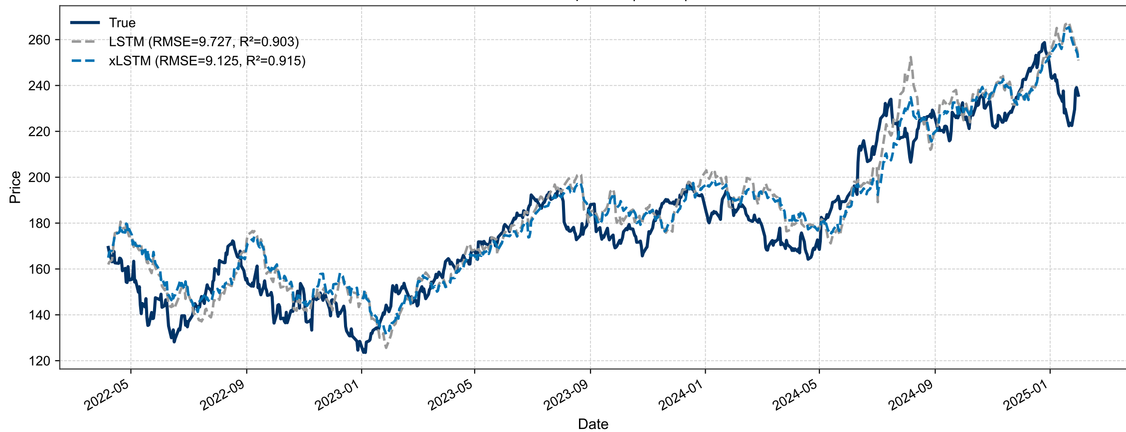
AAPL – Prediction Comparison | H=15 | F=5 – TEST
