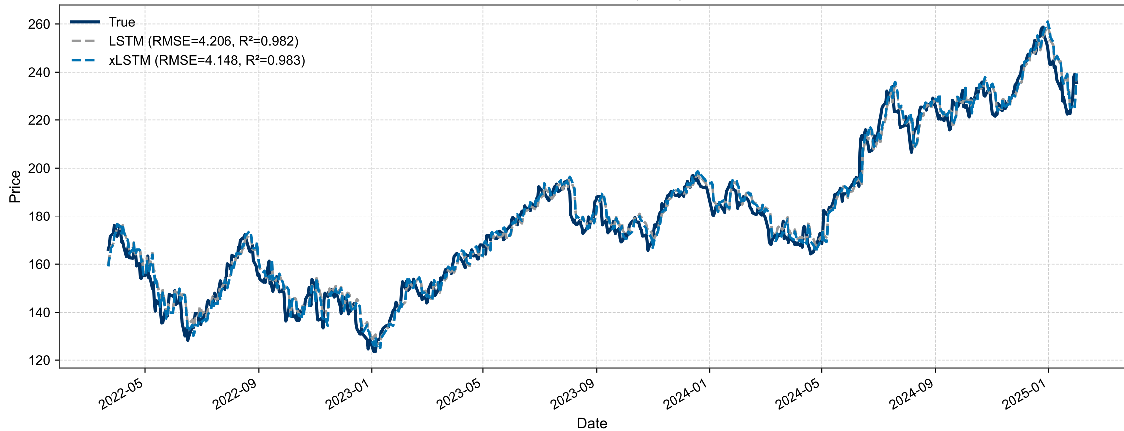
AAPL – Prediction Comparison | H=3 | F=1 – TEST
