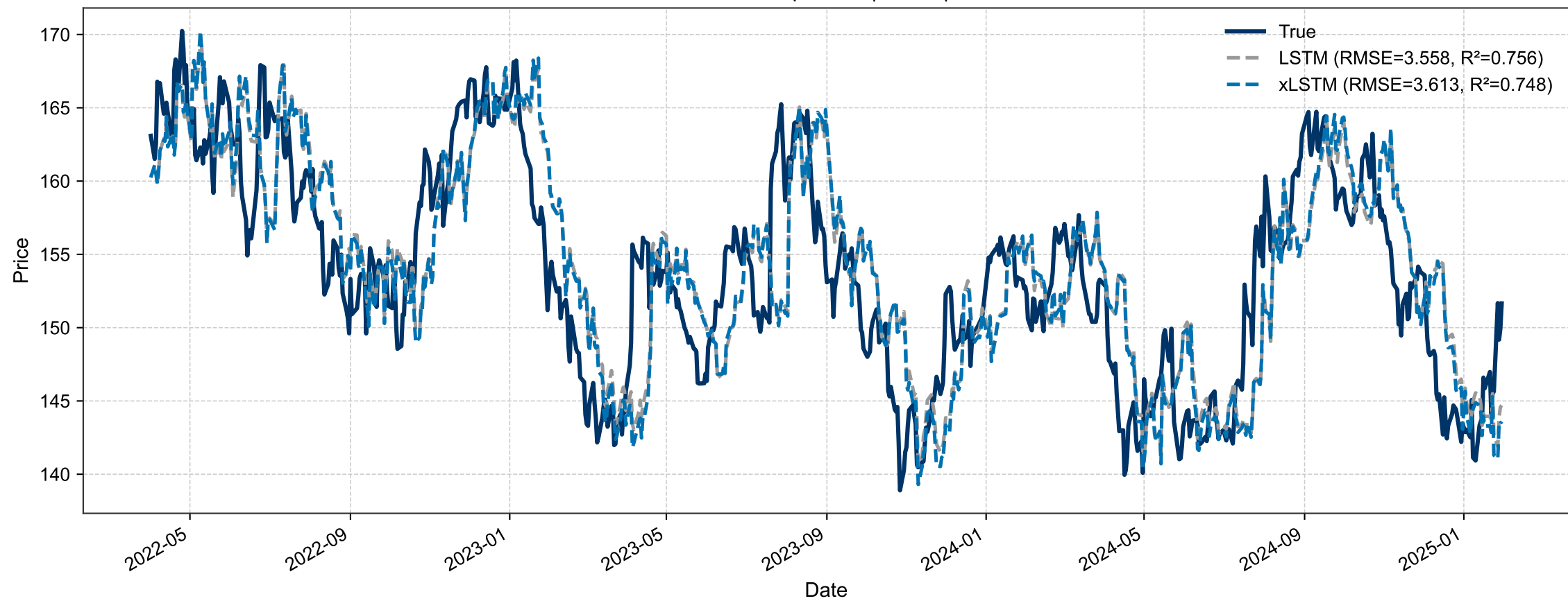
JNJ – Prediction Comparison | H=10 | F=1 – TEST
