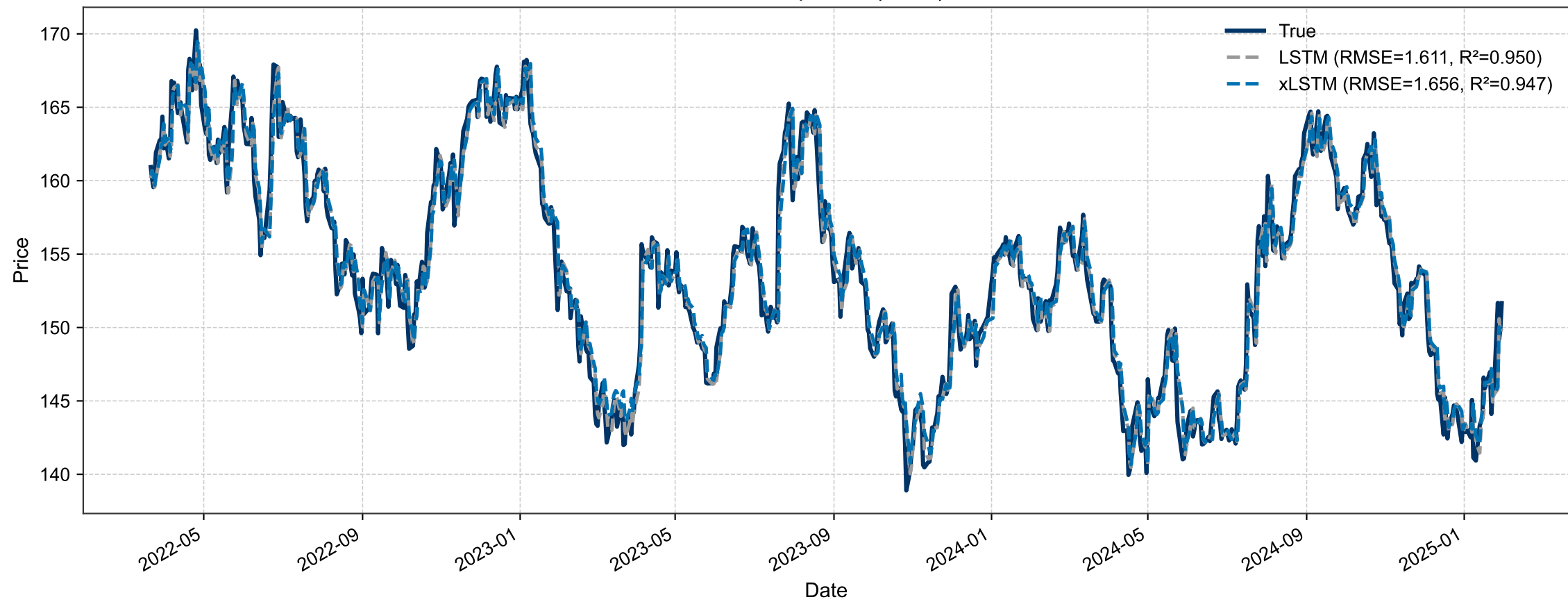
JNJ – Prediction Comparison | H=1 | F=1 – TEST
