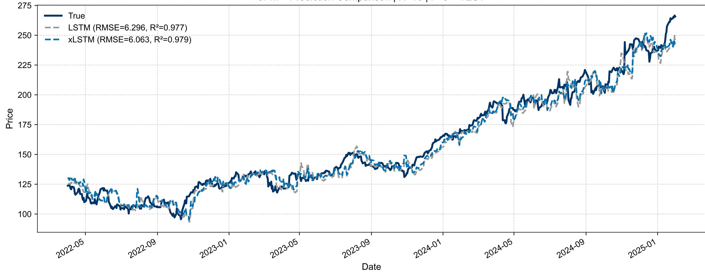
JPM – Prediction Comparison | H=10 | F=5 – TEST
