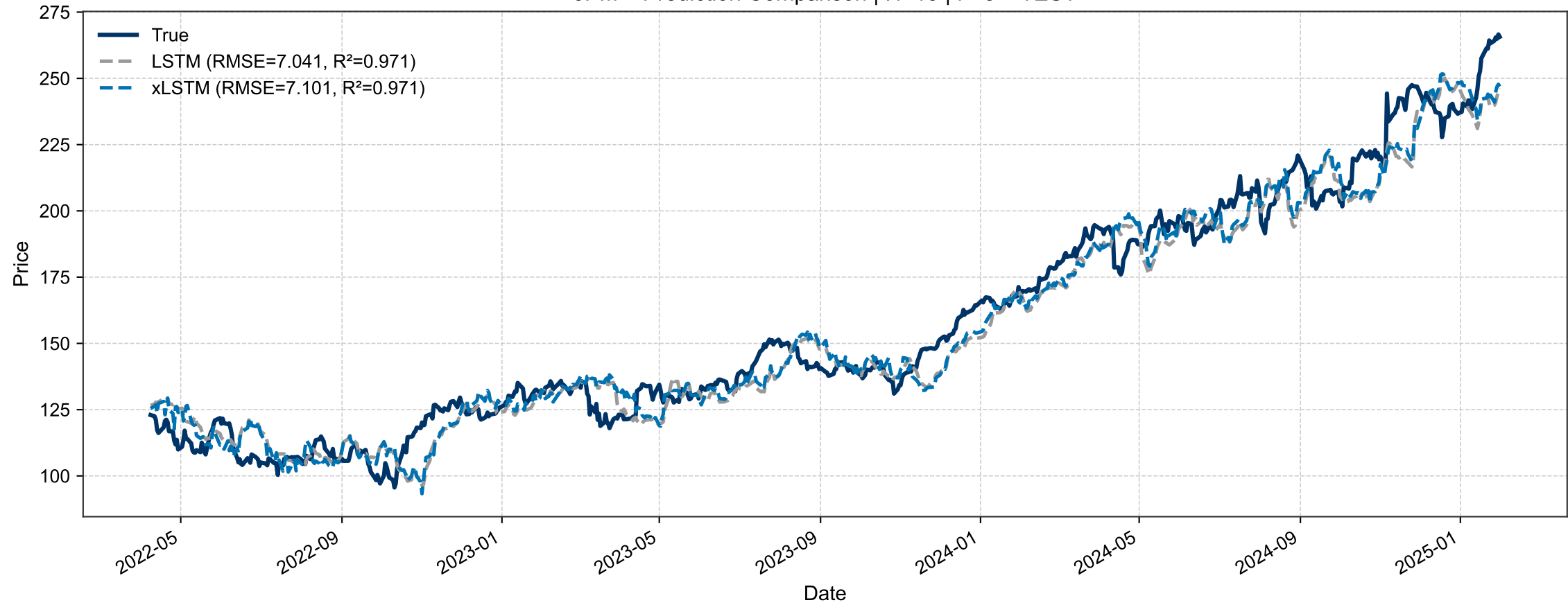
JPM – Prediction Comparison | H=15 | F=5 – TEST
