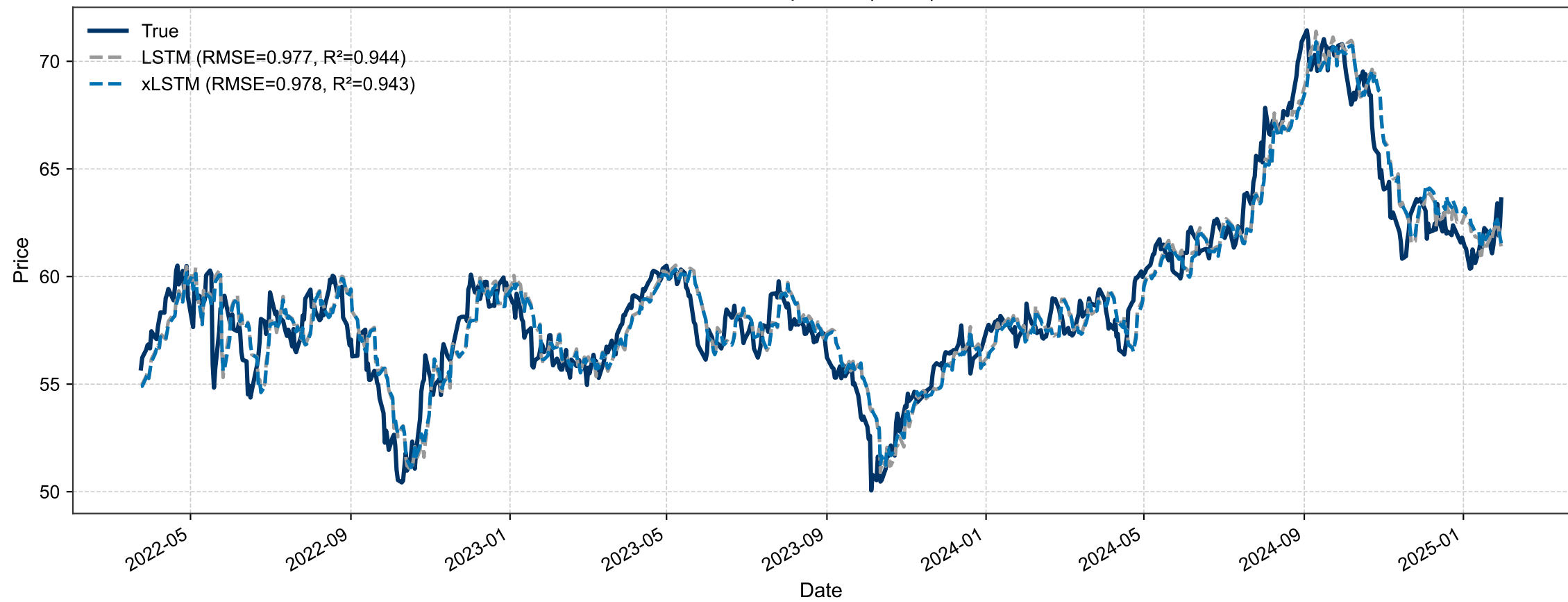
KO – Prediction Comparison | H=5 | F=1 – TEST
