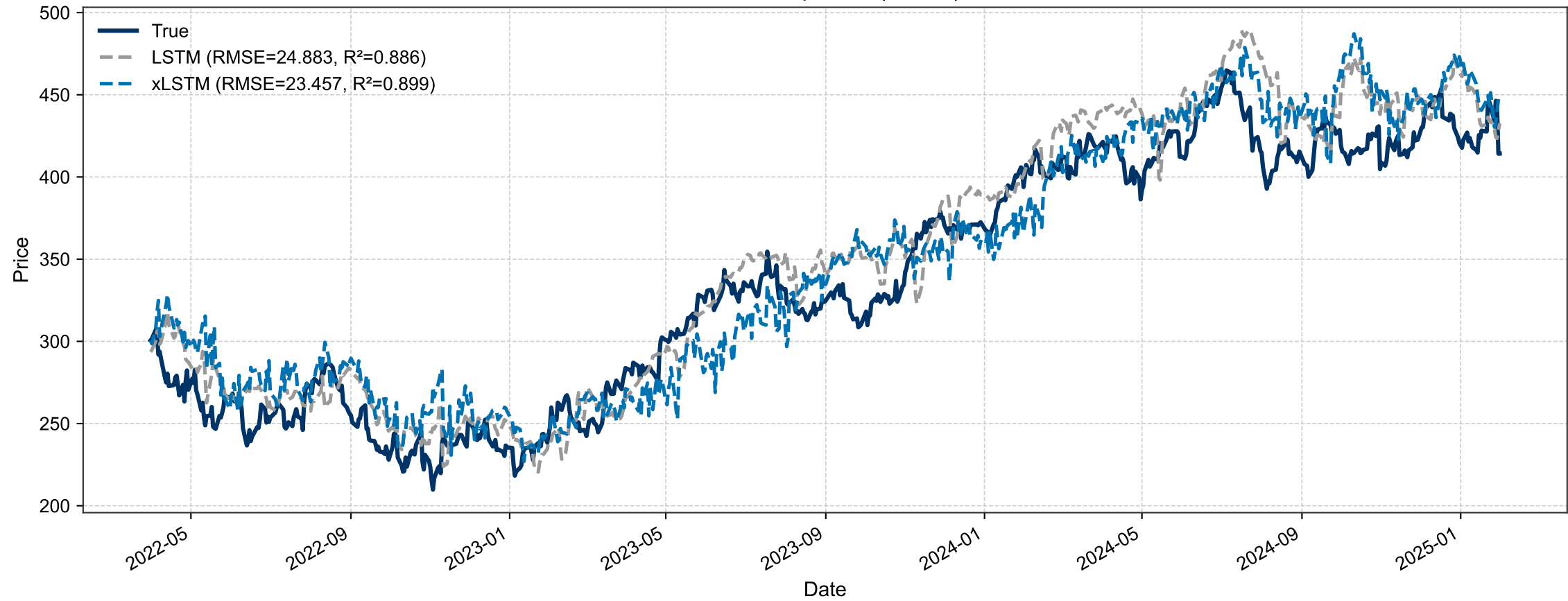
MSFT – Prediction Comparison | H=10 | F=5 – TEST
