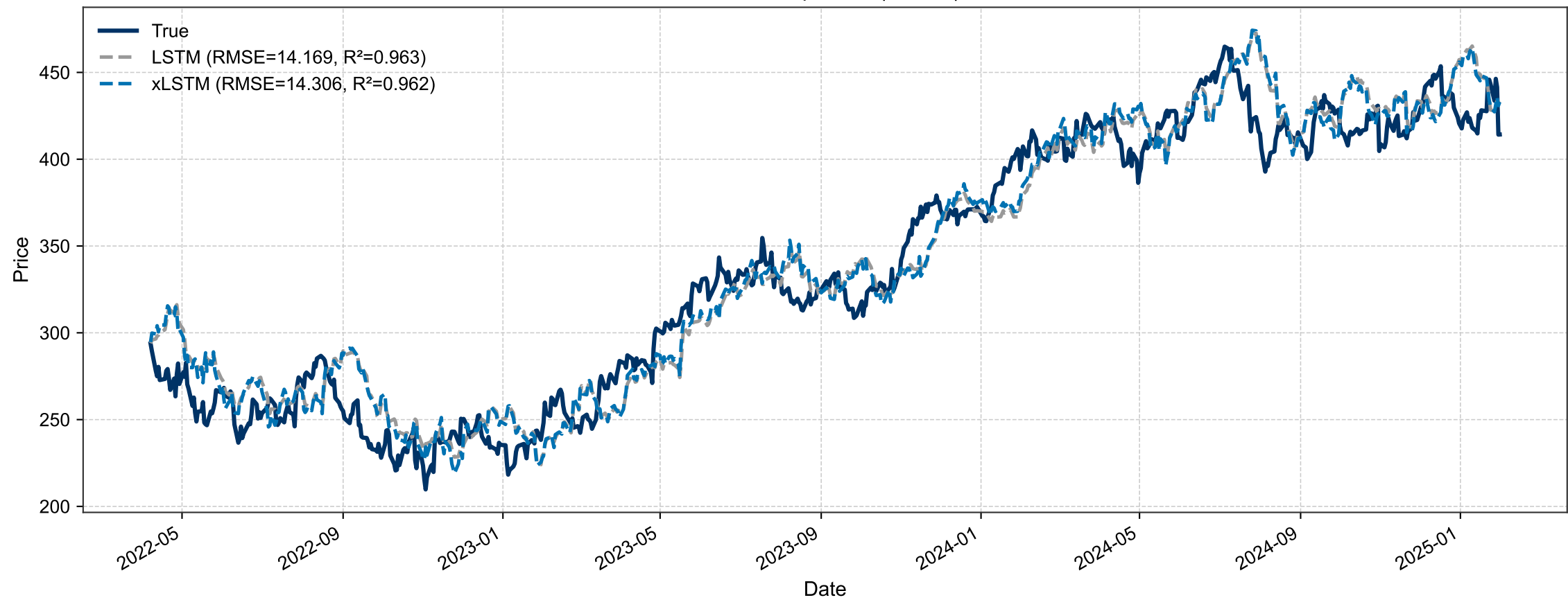
MSFT – Prediction Comparison | H=15 | F=1 – TEST
