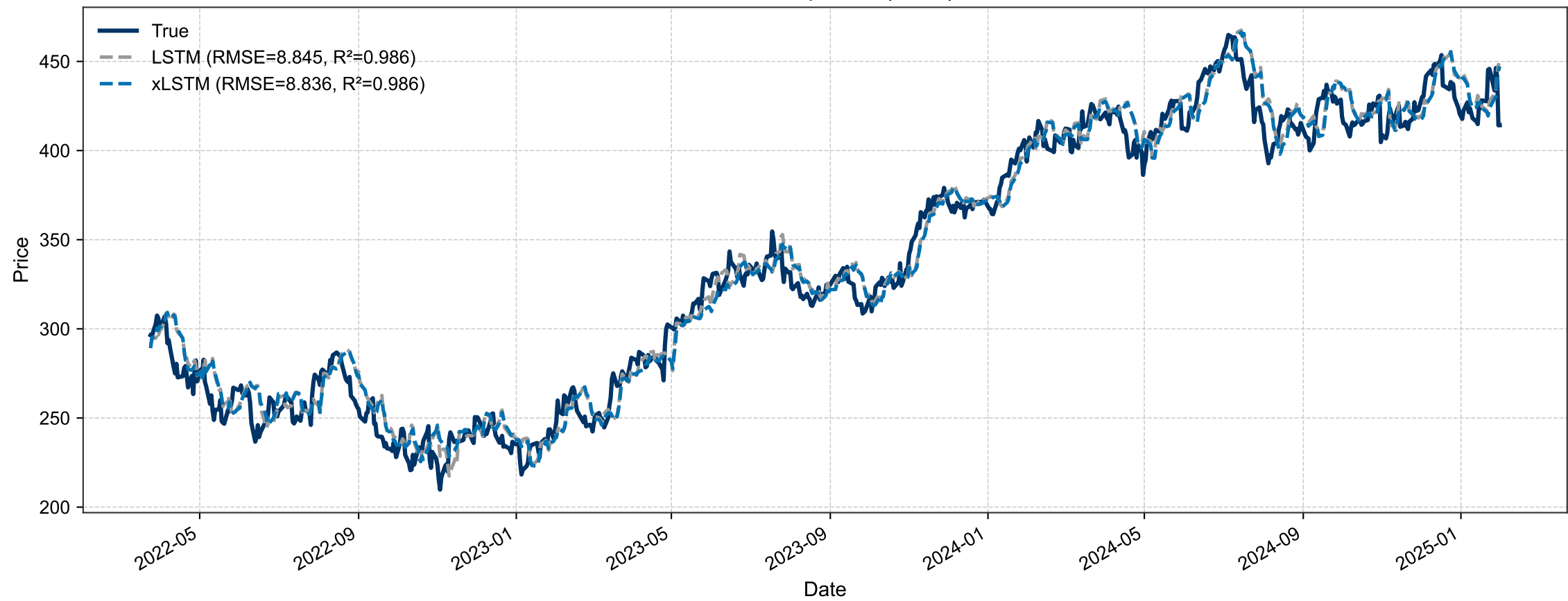
MSFT – Prediction Comparison | H=5 | F=1 – TEST
