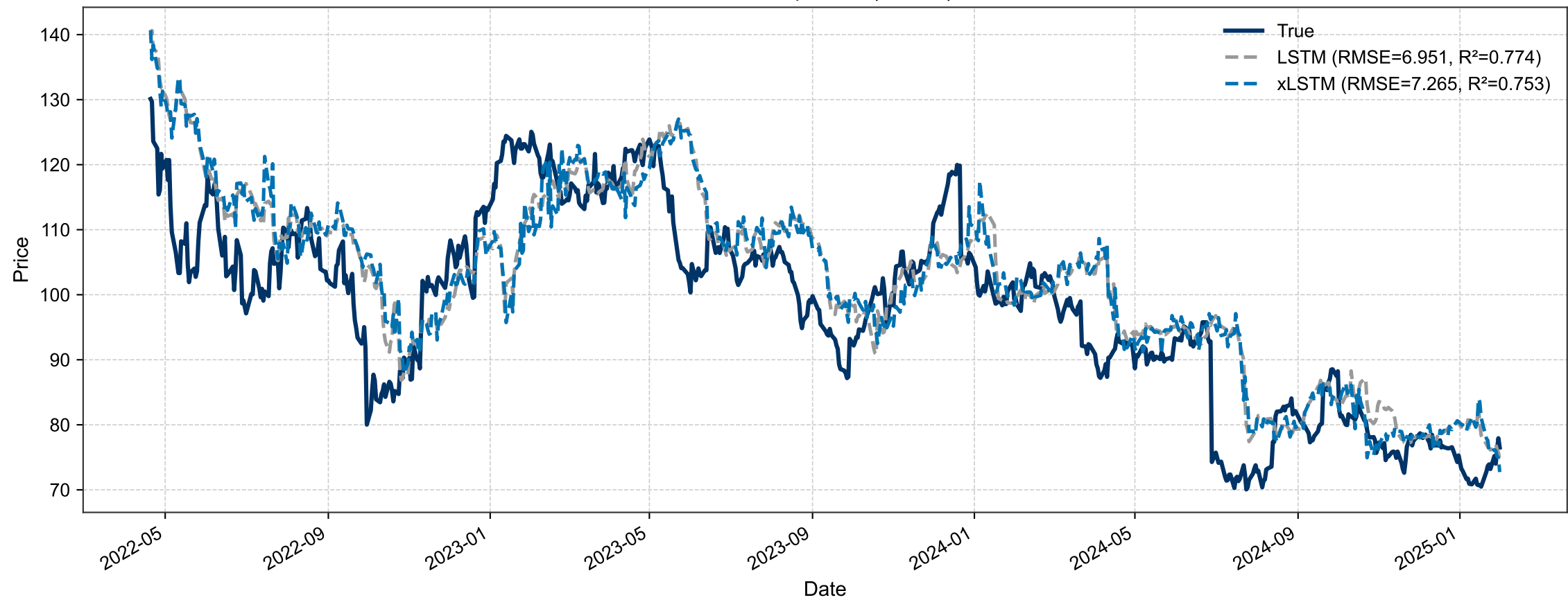
NKE – Prediction Comparison | H=15 | F=5 – TEST
