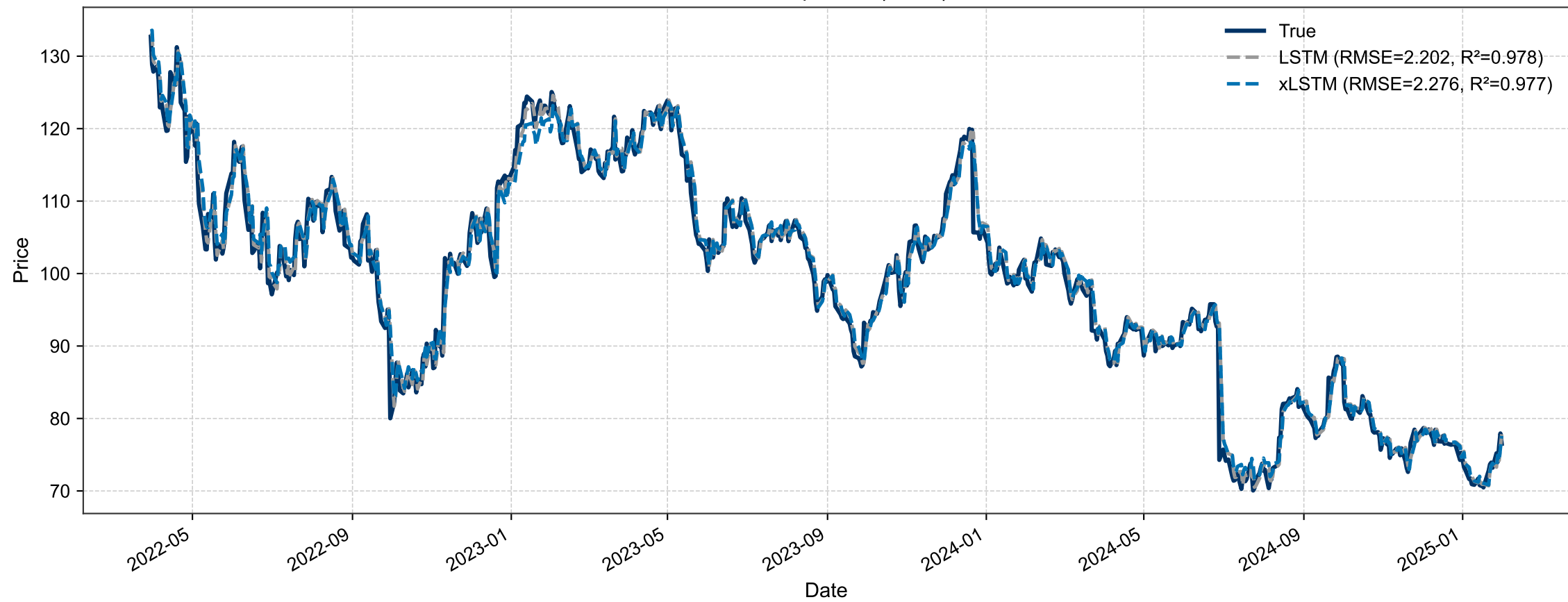
NKE – Prediction Comparison | H=1 | F=1 – TEST
