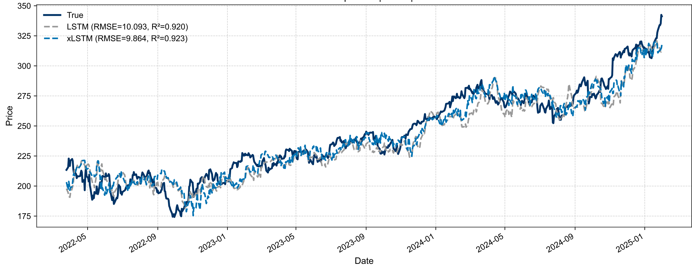
V – Prediction Comparison | H=15 | F=5 – TEST
