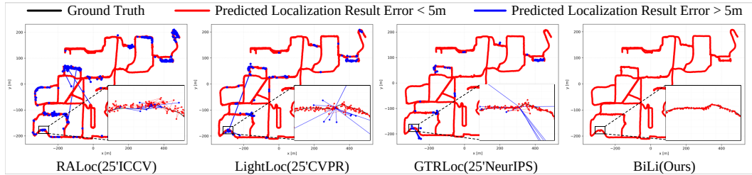
Figure 4: Visualization of localization results on NCLT.
