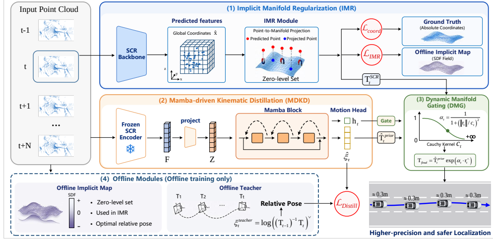
Figure 2: Overview of the proposed BiLi framework. (1) In the spatial domain, IMR constrains representation learning by anchoring absolute predictions to the physical zero-level set via manifold projection. (2) In the temporal domain, MDKD distills offline kinematics into a Mamba block to extract a stable kinematic prior \hat{\mathbf{T}}_t^{\text{prior}} and hidden states \mathbf{h}_t . (3) DMG dynamically fuses the spatial observation \mathbf{T}_t^{\text{SCR}} and the kinematic prior via an \mathbf{h}_t -guided Cauchy kernel. (4) The Offline Modules act as a high-fidelity Teacher, providing spatiotemporal supervision exclusively during training.
