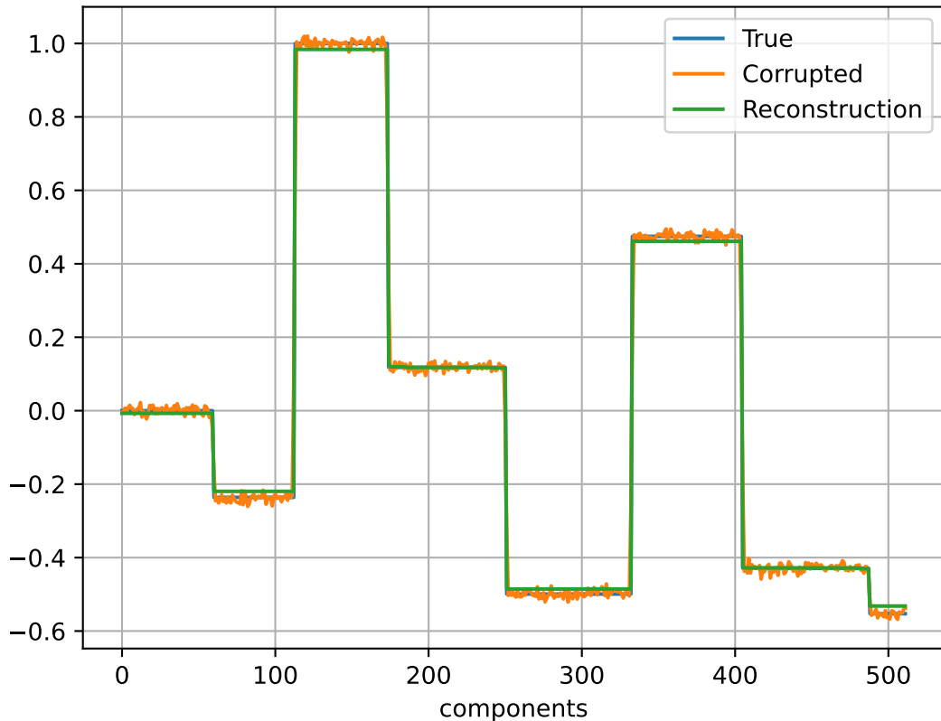
Corrupted vs Reconstruction vs True
