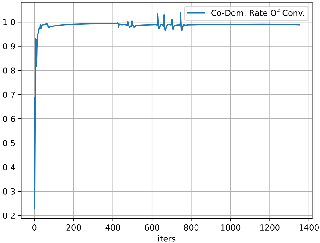
Co-Domain: Rate Of Convergence vs Iters
