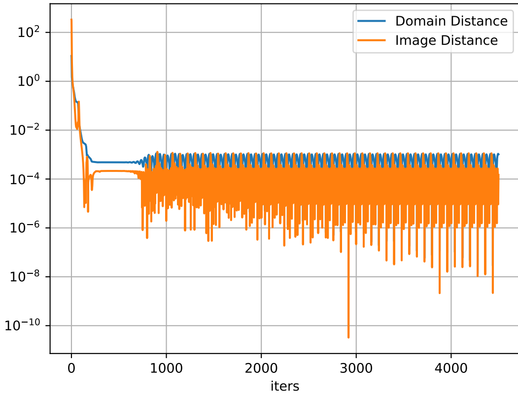
Metrics vs Iters
