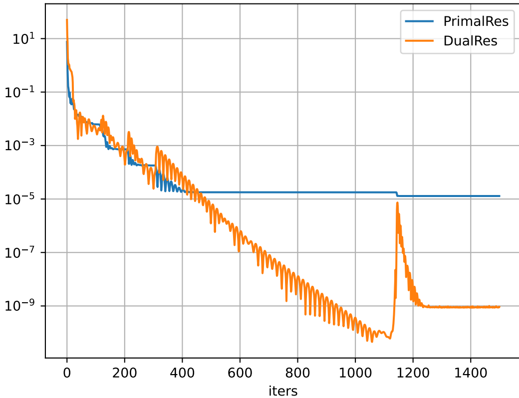
Residuals vs Iters
