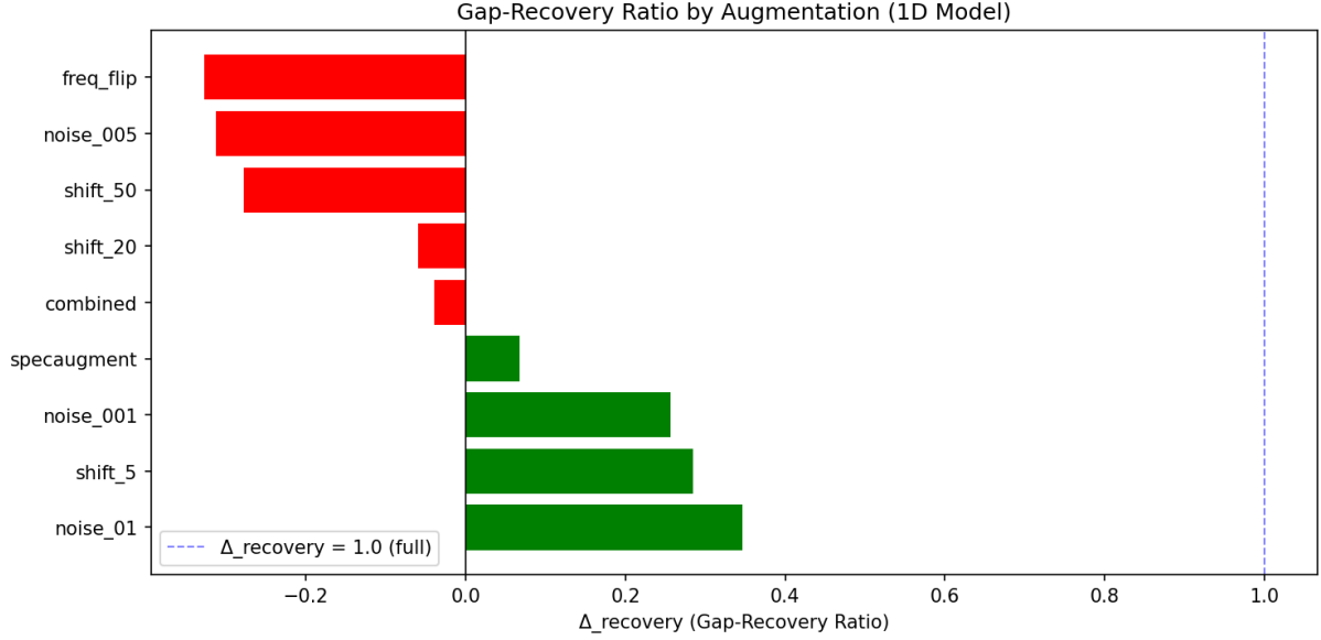
Figure 10: Gap-recovery ratio by augmentation (1D-CNN).
