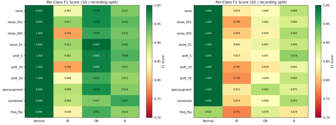
Figure 9: Per-class F1 heatmaps. Left: 1D-CNN. Right: 2D-CNN.
