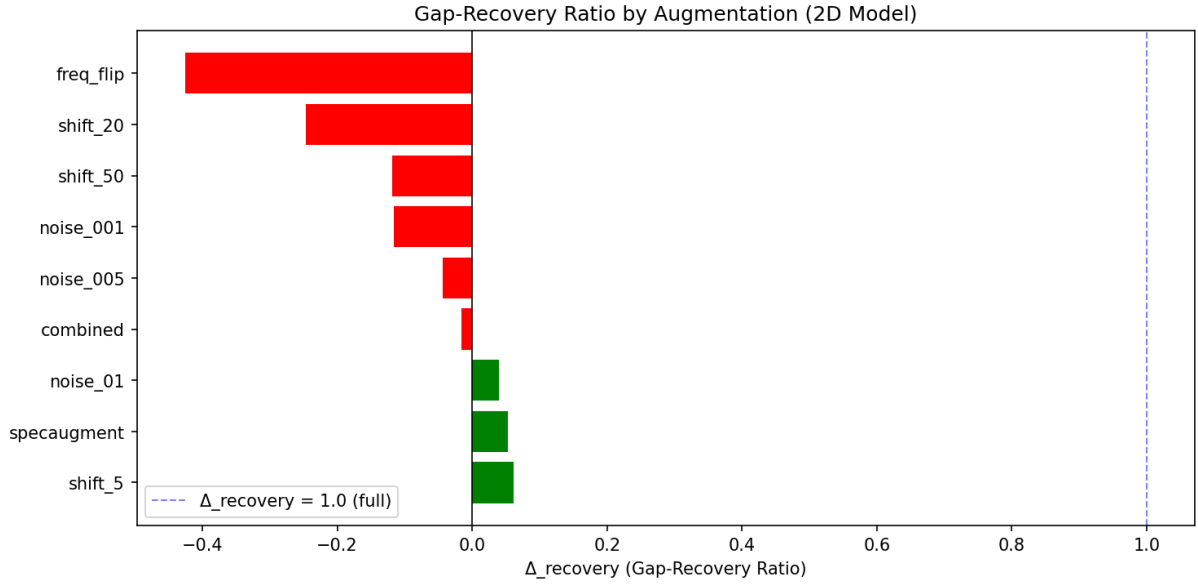
Figure 11: Gap-recovery ratio by augmentation (2D-CNN).
