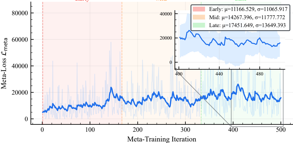
Training Phase Analysis with Convergence Zoom
