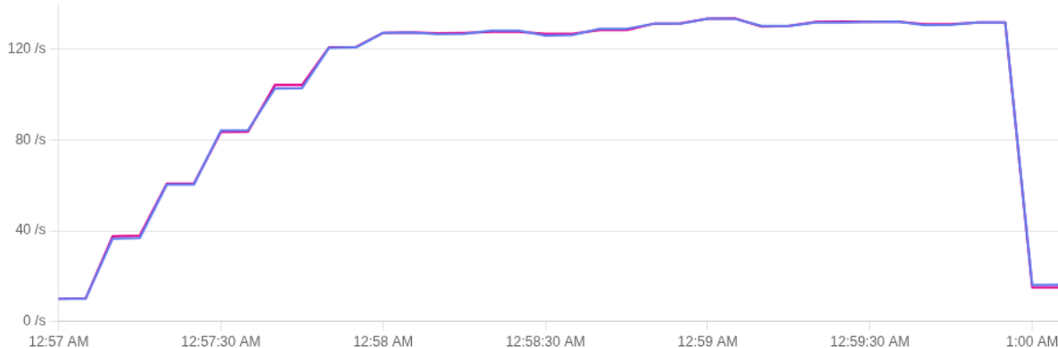
Requests/sec (avg)
