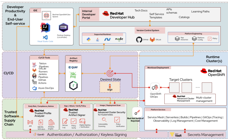
Figure 4. Application Platform Tools(Click the image to view it in full size in a new browser tab)
