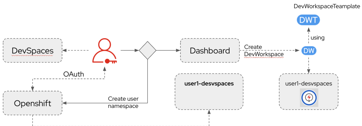
Figure 17. Workspace Creation Workflow(Click the image to view it in full size in a new browser tab)
