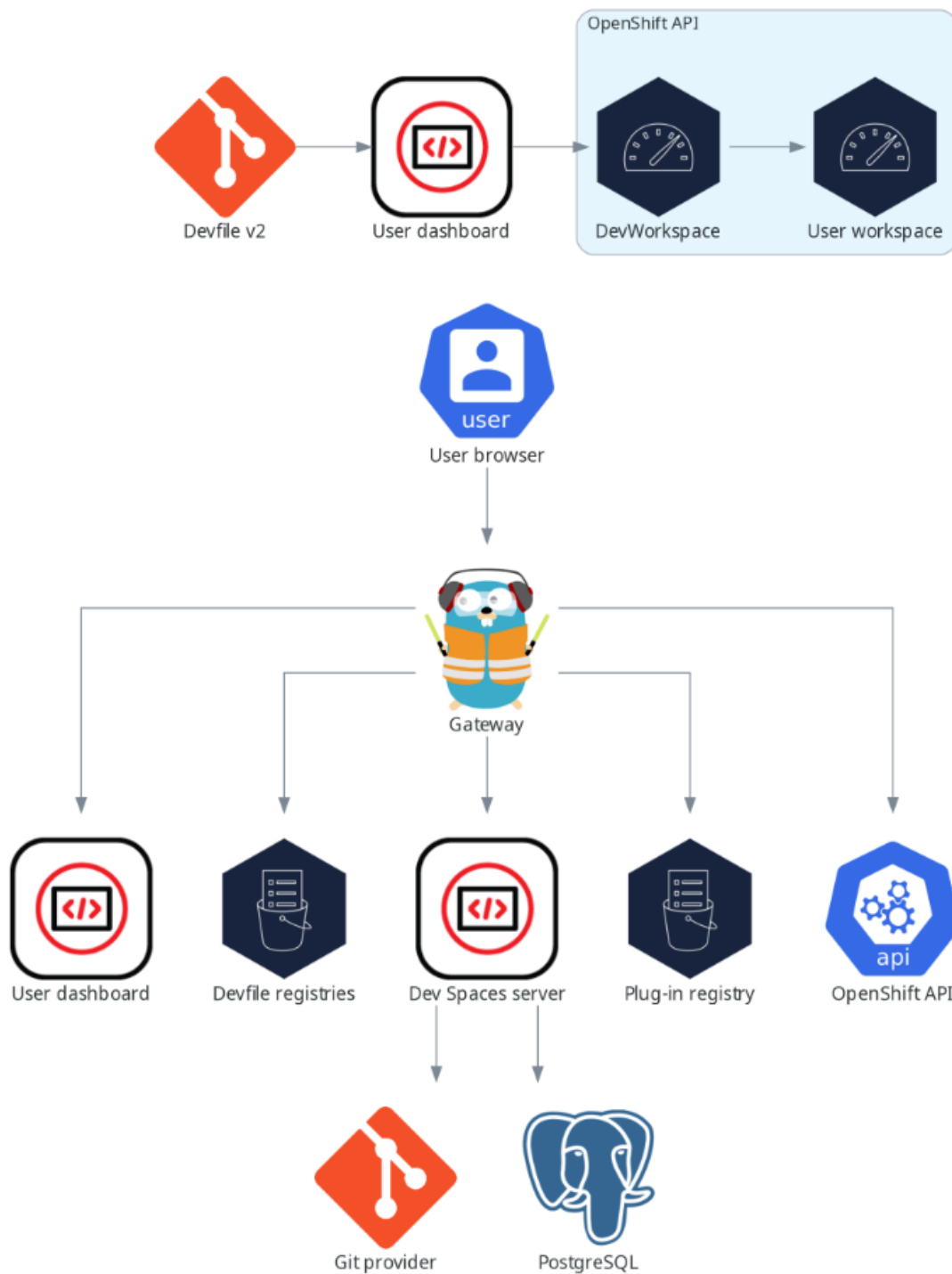
Figure 13. DevSpaces Architecture(Click the image to view it in full size in a new browser tab)
