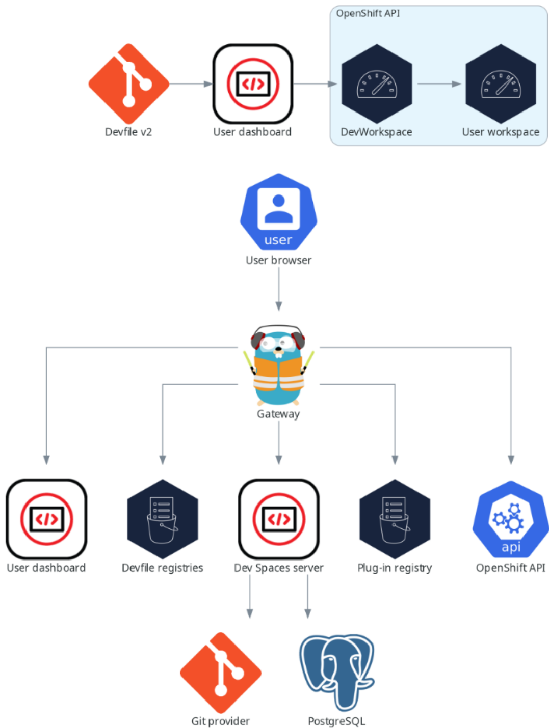
Figure 24. DevSpaces Architecture(Click the image to view it in full size in a new browser tab)
