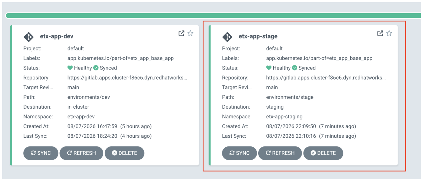
Figure 35. ArgoCD Application status
