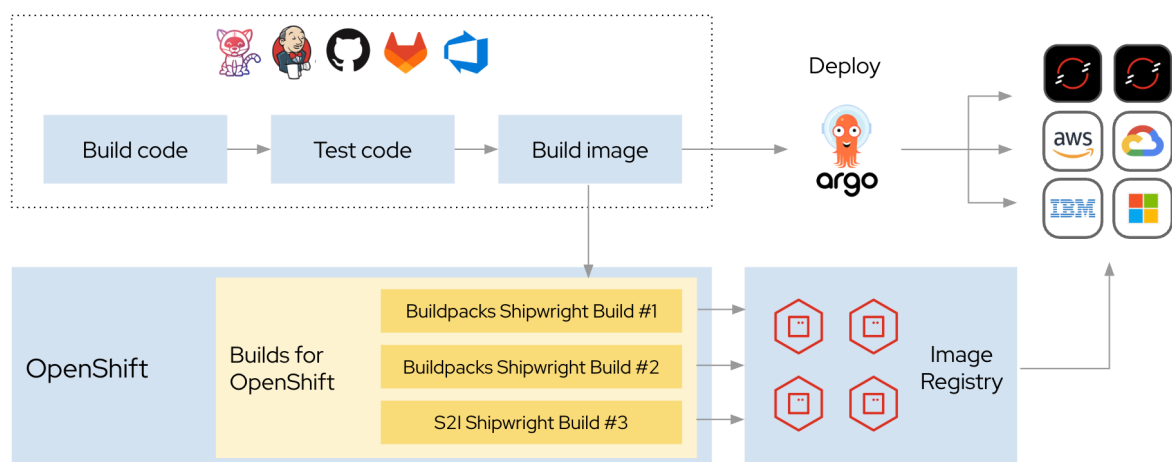
Figure 2. OpenShift image build workflow(Click the image to view it in full size in a new browser tab)
