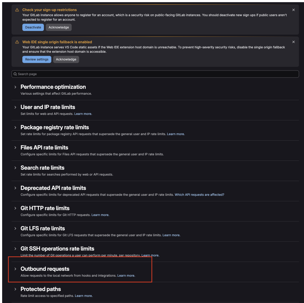
Figure 6. Outbound Requests(Click the image to view it in full size in a new browser tab)
