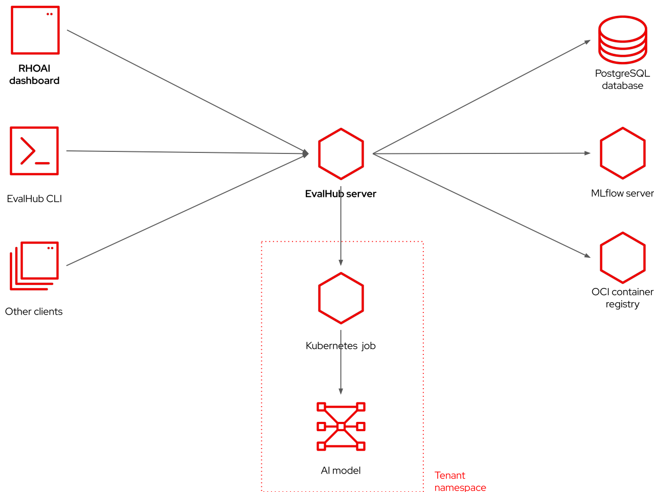
Figure 2. Architecture of EvalHub
