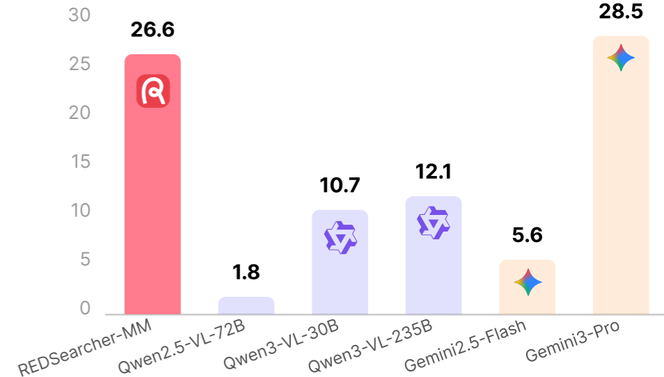
BrowseComp-VL
