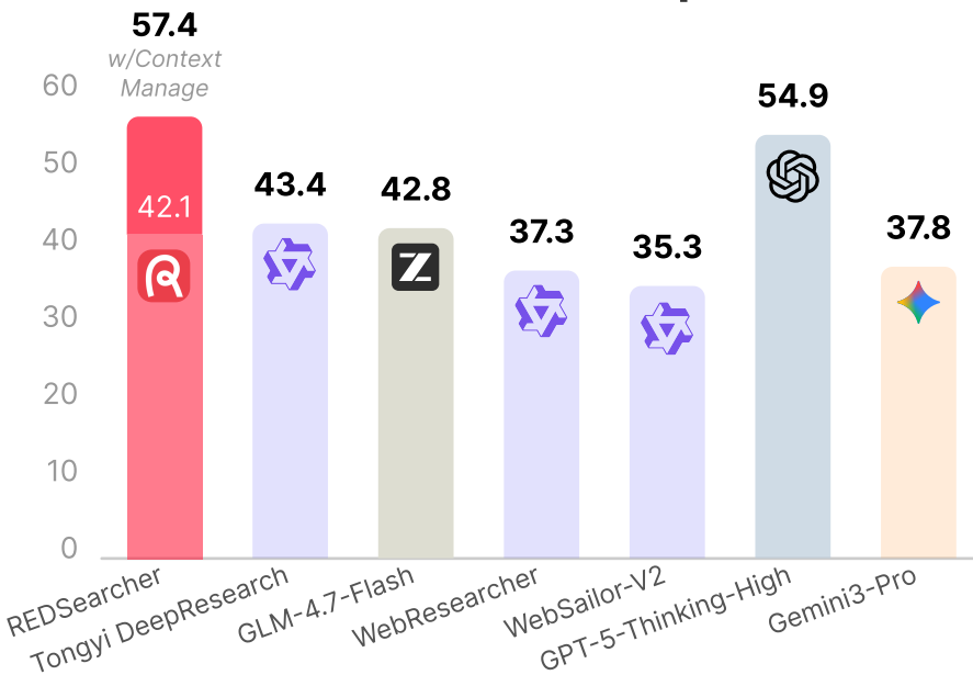
BrowseComp
