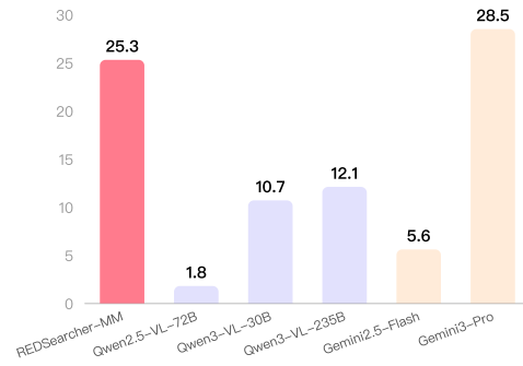
BrowseComp-VL
