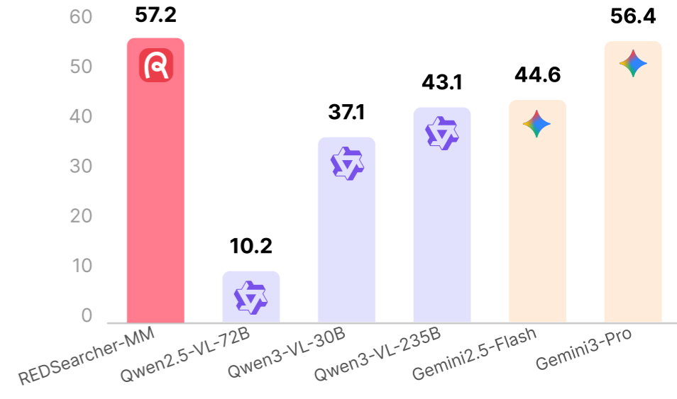
BrowseComp-VL
