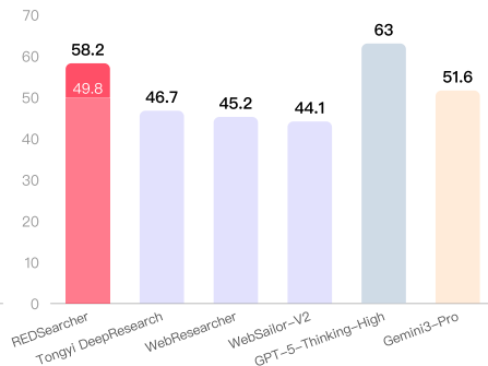
GAIA
