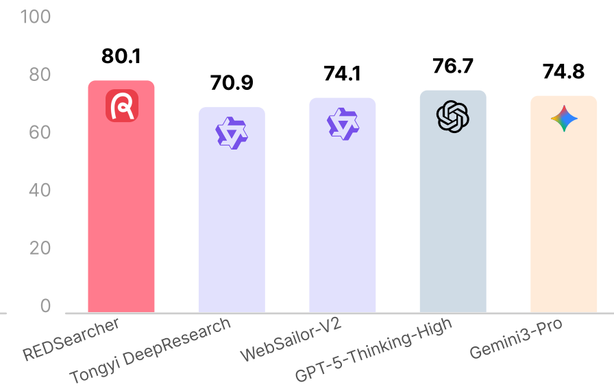
GAIA
