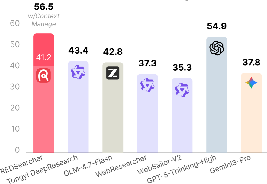
BrowseComp
