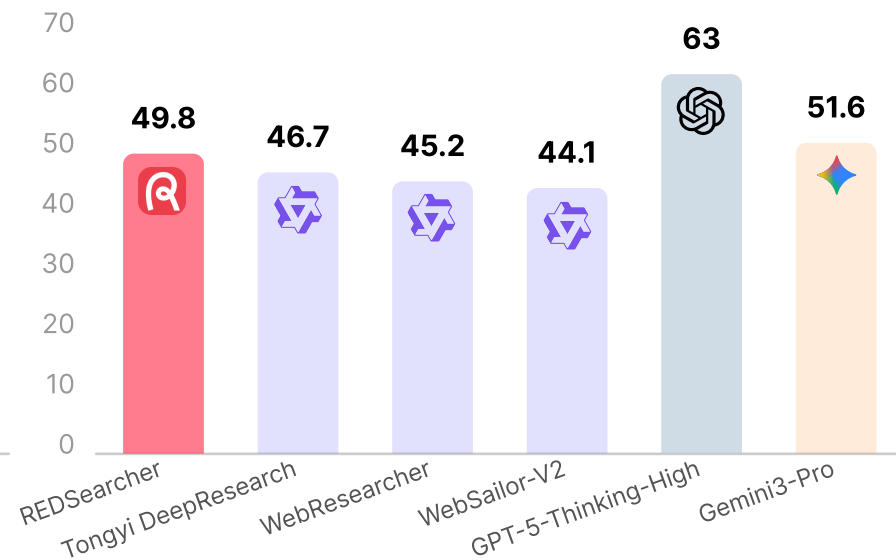
GAIA
