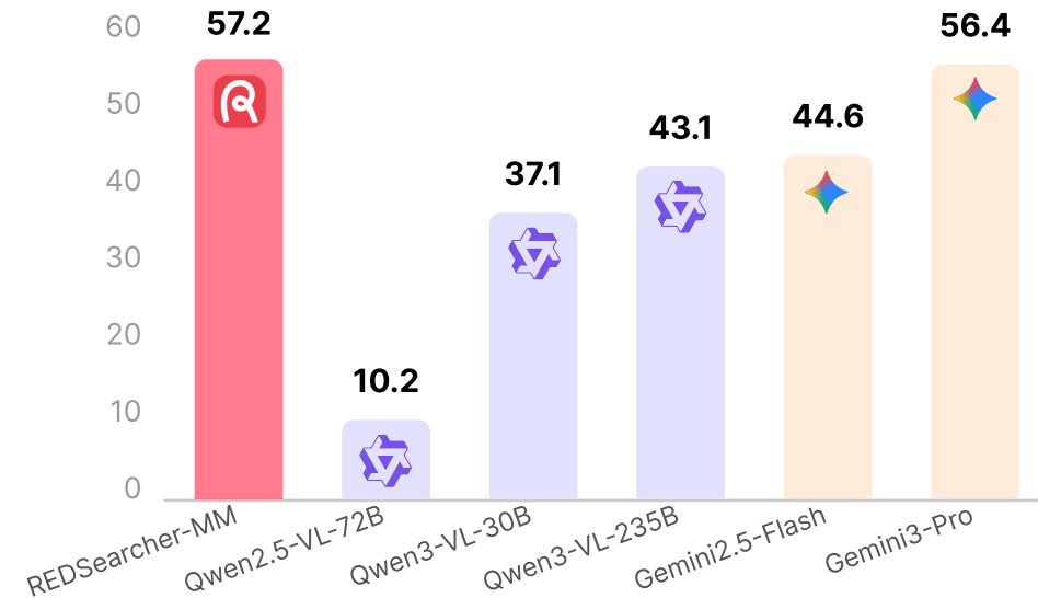
BrowseComp-VL
