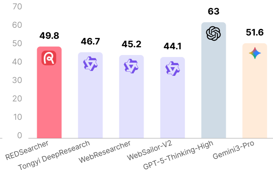
GAIA
