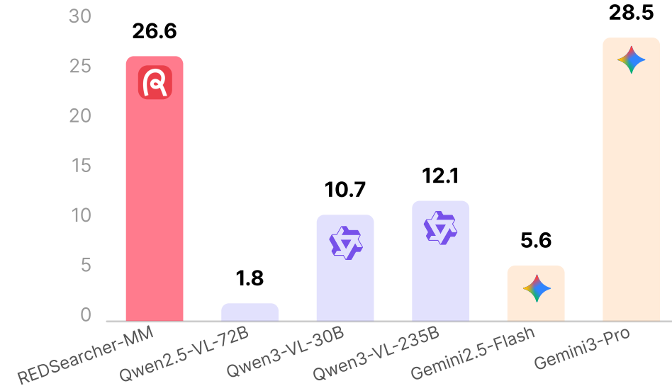
BrowseComp-VL
